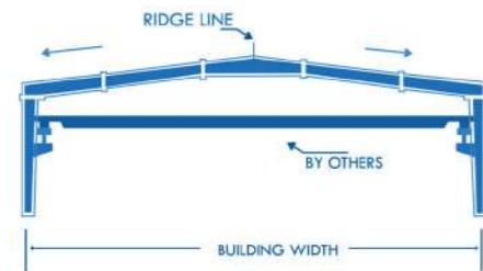
Clear Span with Crane
