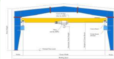
Top Running Crane
