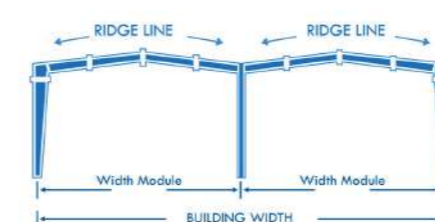
Mutli Gable (MG) I-II
