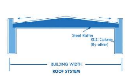
Rafter System
