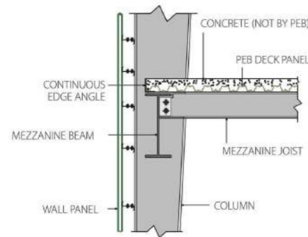
Mezzanine Joist Connection to Mezzanine Beam
