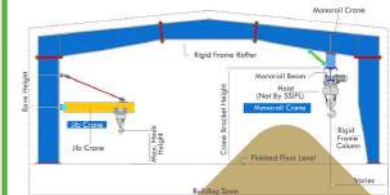
JIB and MonoRail Crane
