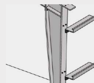
Wall Girts
