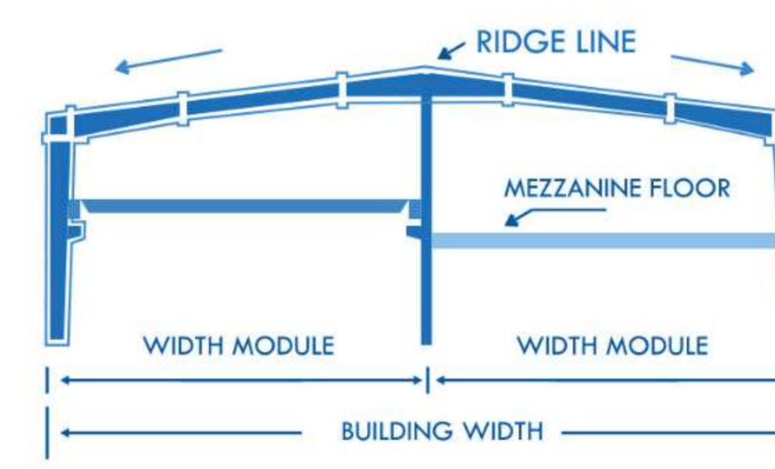
Multi Span With Crane and Mezzanine
