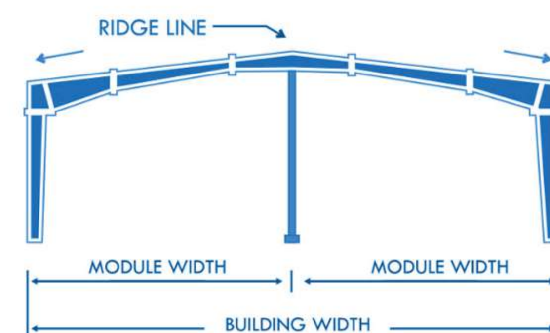
Multi Span I
