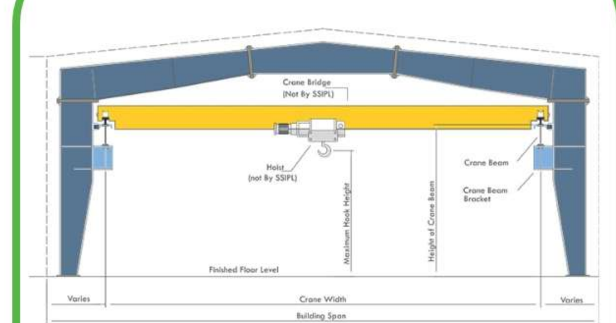
Top Running Crane
